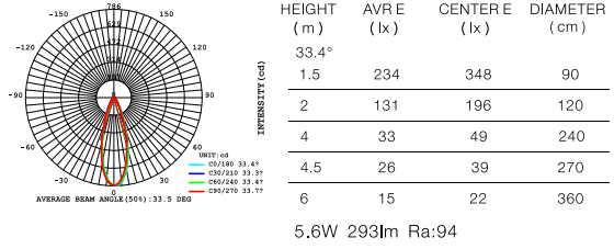
LED 3000K CODE:AA8888888
